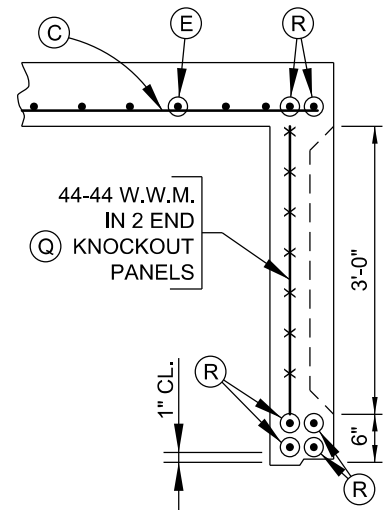
SECTION 2-2
